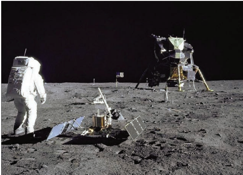
Figure 2.4: Lunar Surface
