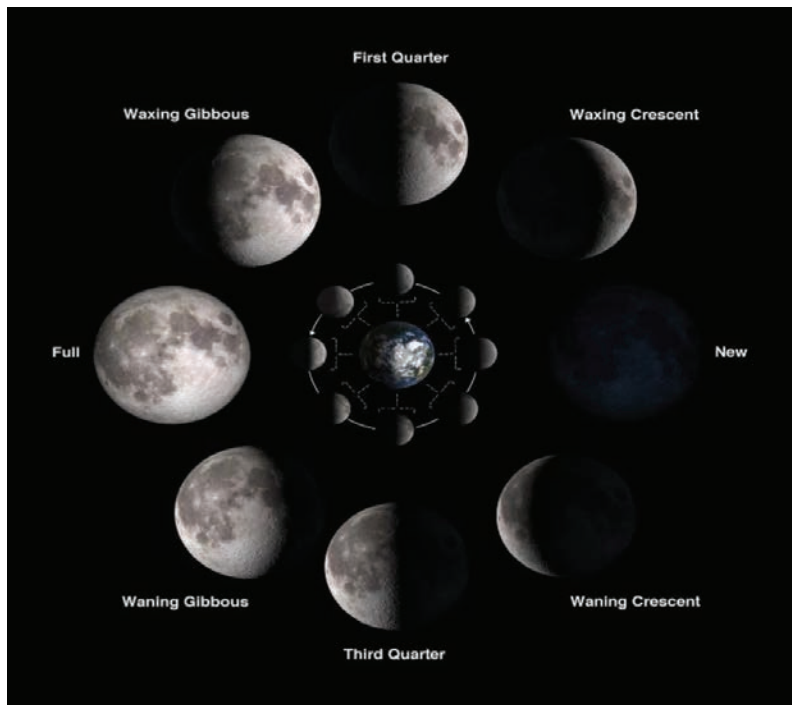
Figure 2.6: Phases of Moon (Credit: NASA/Bill Dunford)
