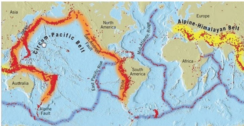
Figure 1.21: Seismic zones of the world
