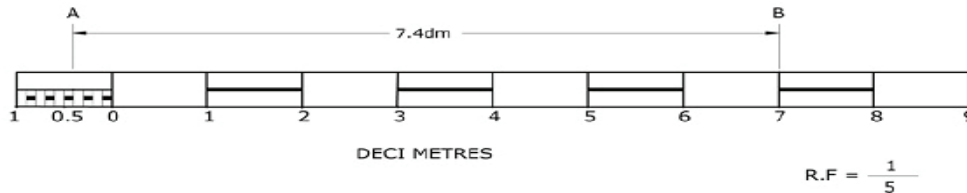
Figure 3.8: Plain Scale
