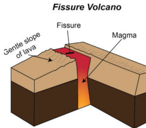
Figure 1.4: Fissure type
